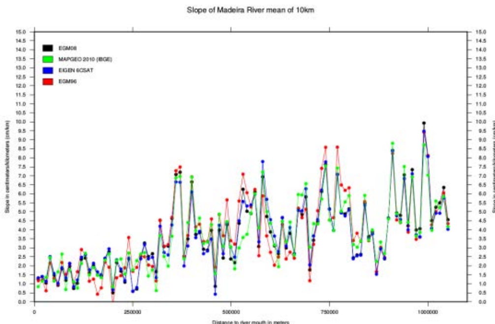
Figure 60. Longitudinal derivative of a GPS profile of the free surface of the Madeira river (averaged every 10 km), using different geoid models. Note that the major undulations exhibited by the slope profile are not significantly altered by the choice of the geoid model.
